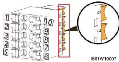
Figure 6-13 Signal cable ports
