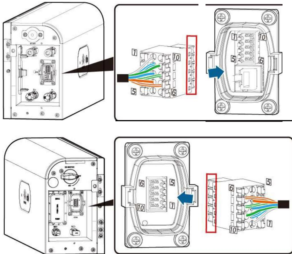
Figure 6-17 Inserting the terminal
