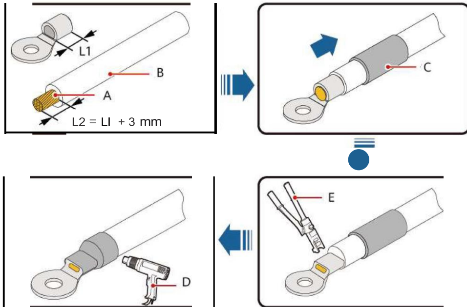
Figure 6-9 Crimping an OT terminal
