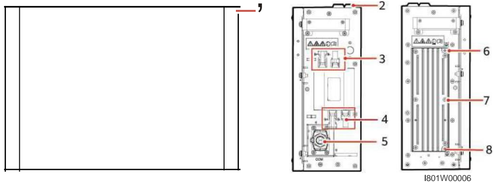
Figure 2-8 Battery expansion module
