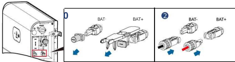
Figure 6-12 Connecting battery cables
