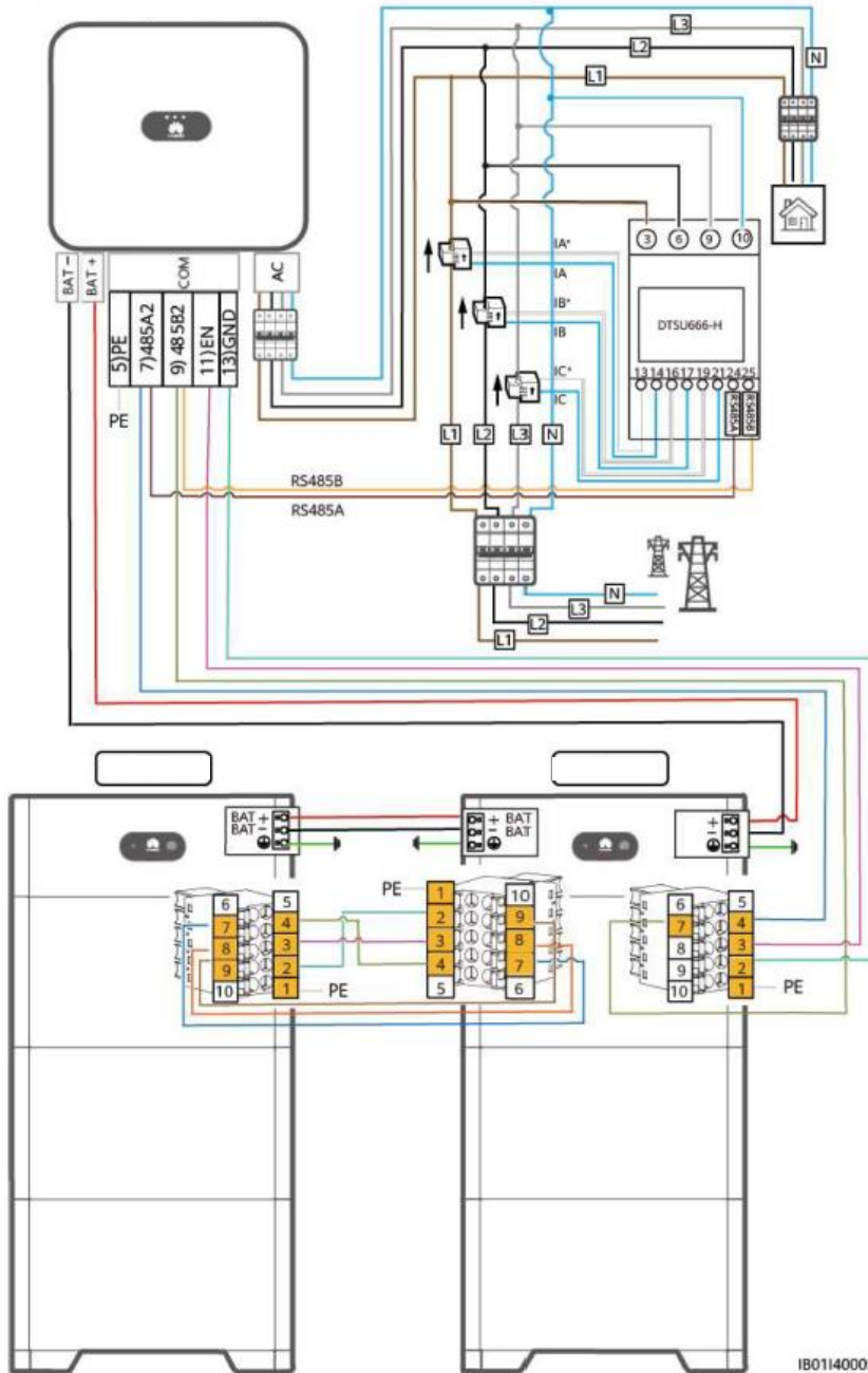
Figure 6-7 Power Shifter 6/8/10kW
