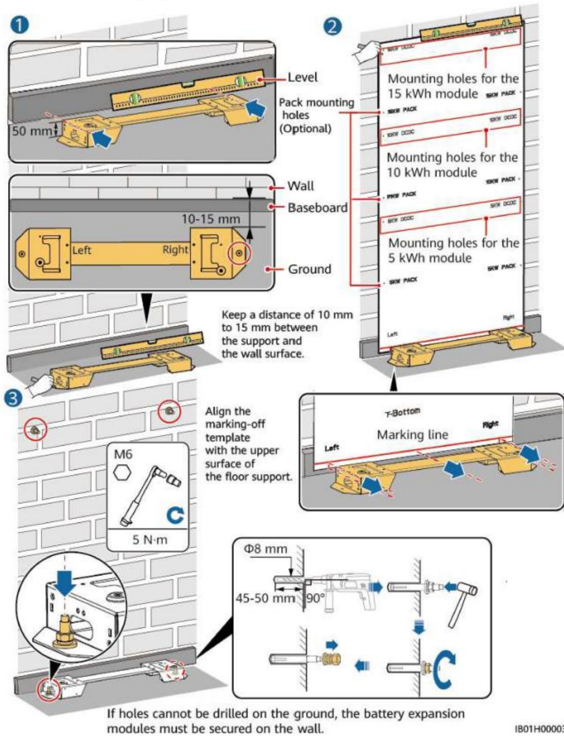
Figure 5-4 Installing expansion bolts
