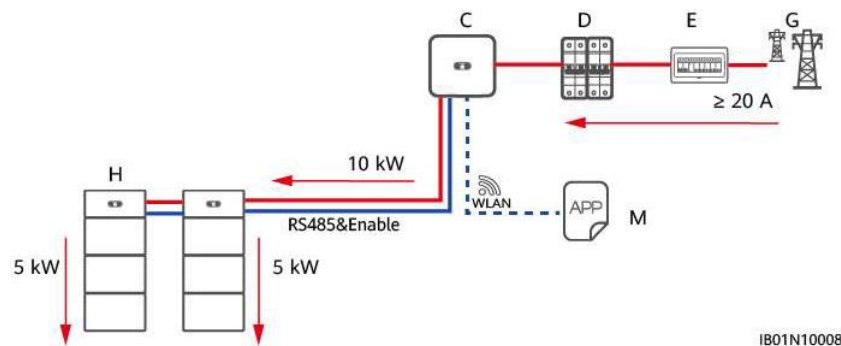
Figure 8-1 Networking diagram for three-phase power supply scenario
