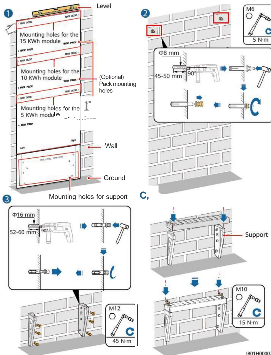
Figure 5-8 Wall-mounted installation
