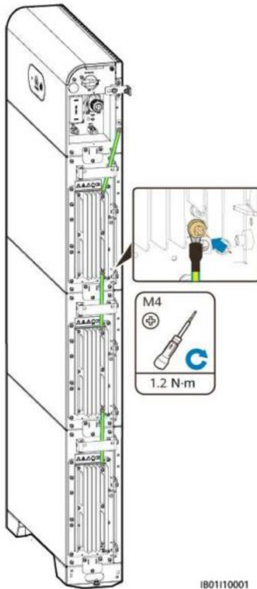
Figure 6-2 Connecting the internal PE cable
