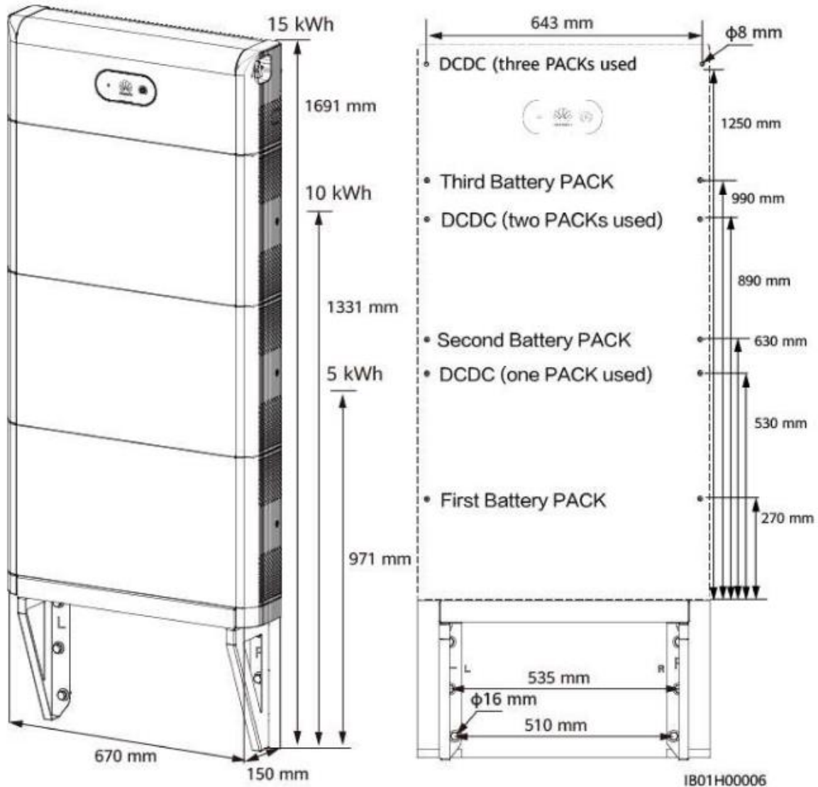
Figure 5-7 Wall-mounted installation dimensions
