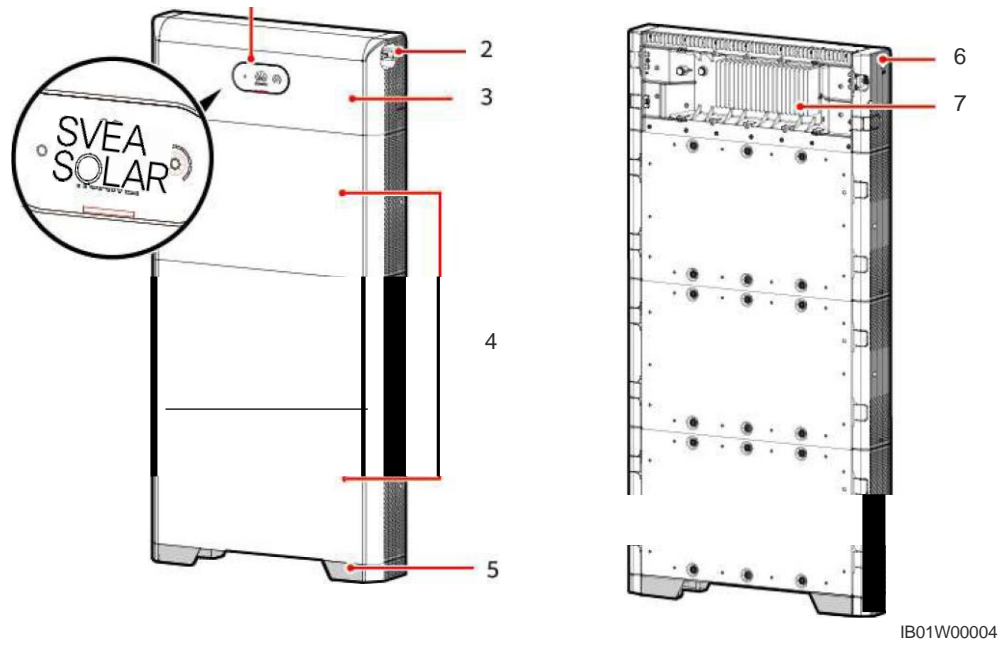
Figure 2-6 Battery appearance
