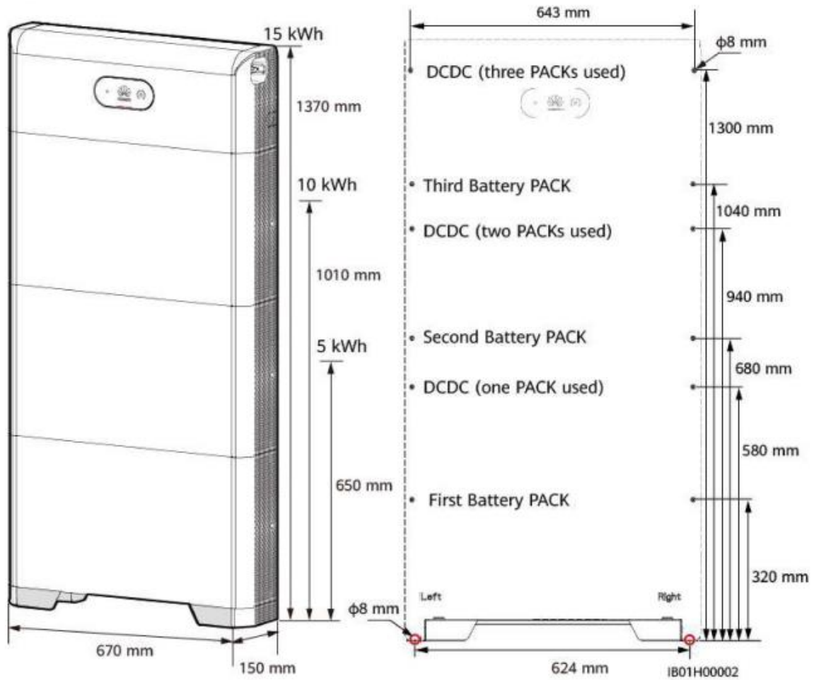
Figure 5-2 Floor-mounted installation dimensions
