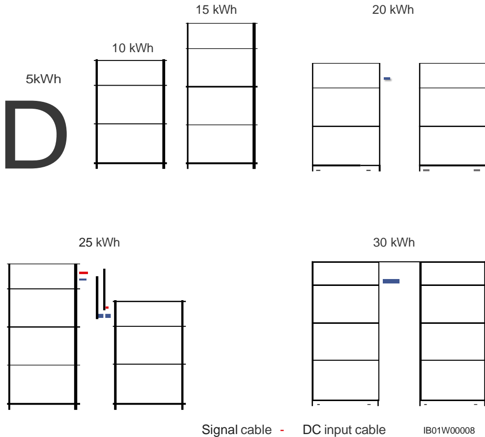
Figure 2-4 Battery capacity description
