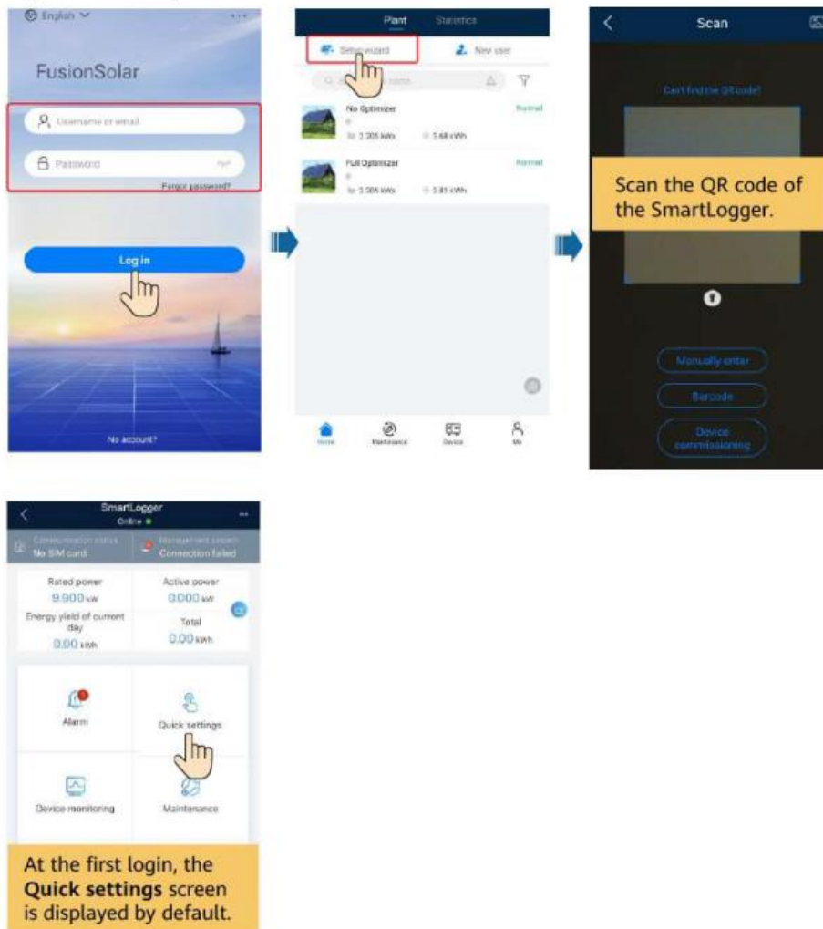
Figure 7-8 Setup Wizard
