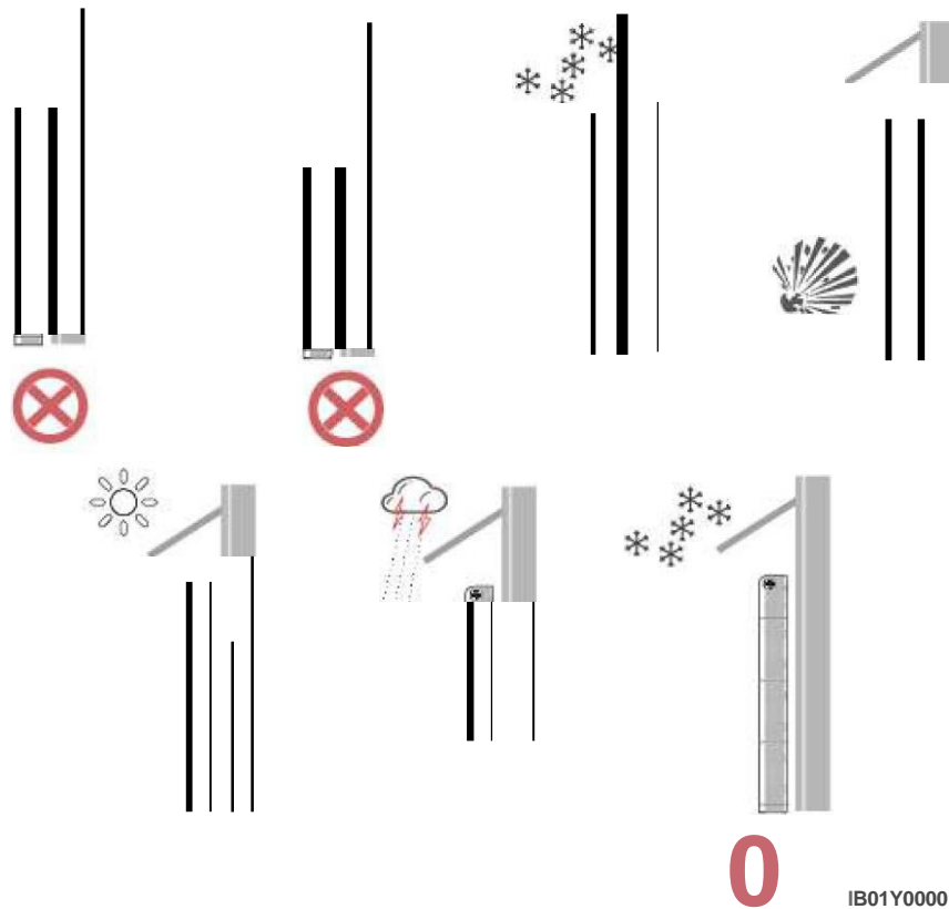
Figure 1-3 Installation environment
