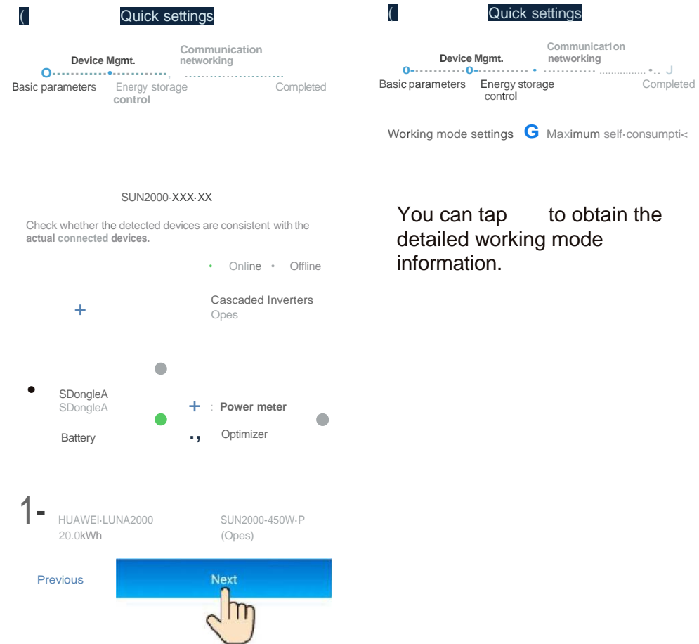
Figure 7-5 Quick settings
