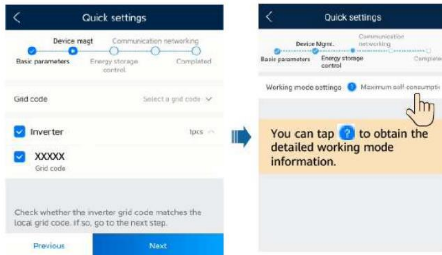
Figure 7-9 Quick settings
