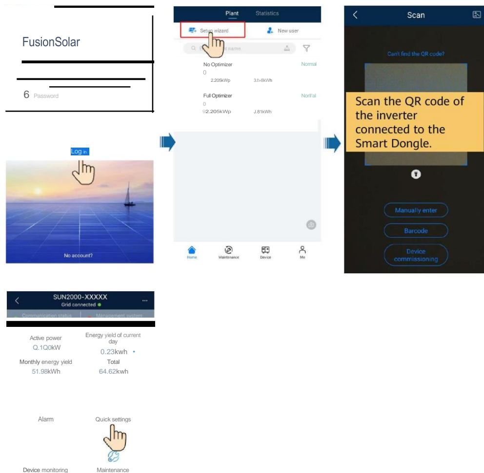
Figure 7-4 Setup Wizard
