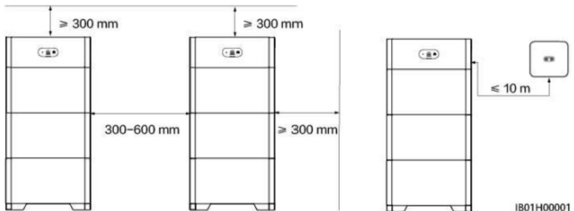
Figure 5-1 Installation space
