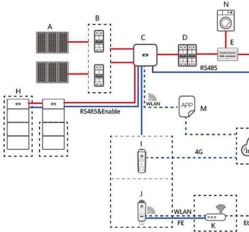
Figure 2-5 Networking (dashed boxes indicate optional components)
